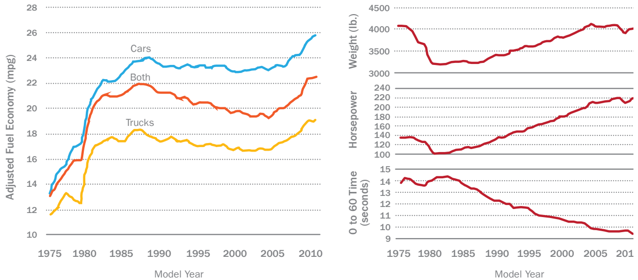
Figure 8. Light-Duty Vehicle Fuel Economy Trends: 1975–2010
