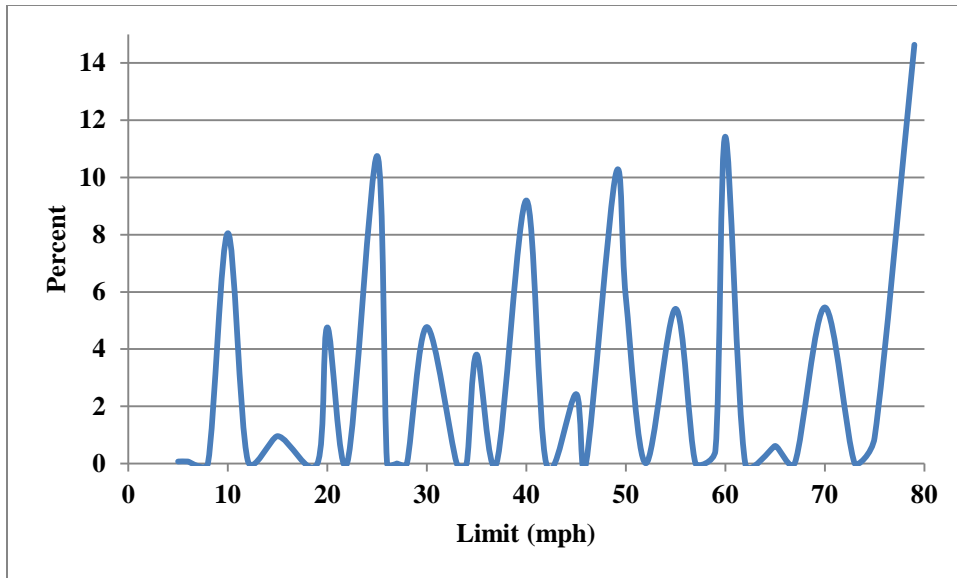
Figure 3.3 Profile of Railroad Speed Limits in the United States
