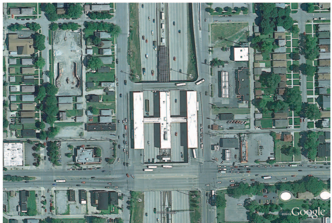
Exhibit 9-14. Example bus station located over rapid transit line (Chicago, Illinois).
