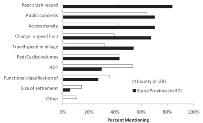
FIGURE 37 Conditions that may prompt more than standard treatment of the transition zone.
