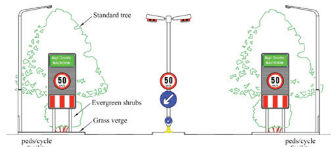
FIGURE 34 Typical gateway landscaping [Source: National Roads Authority (2005)].
