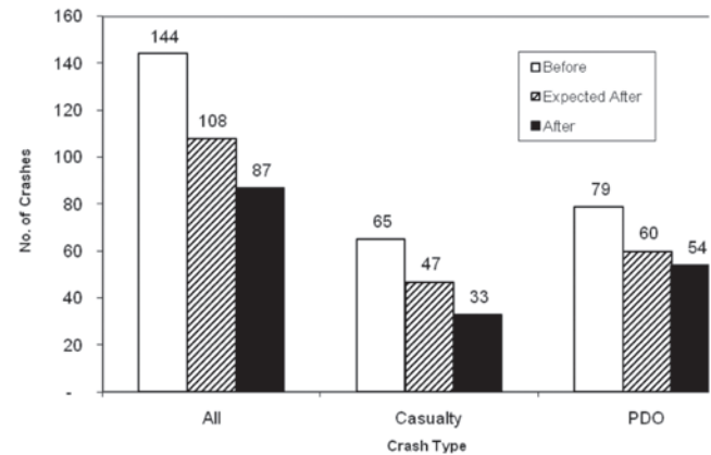
FIGURE 19 Effect of environmentally adapting through roads on crash occurrence [Source: Agustsson (2005)].
