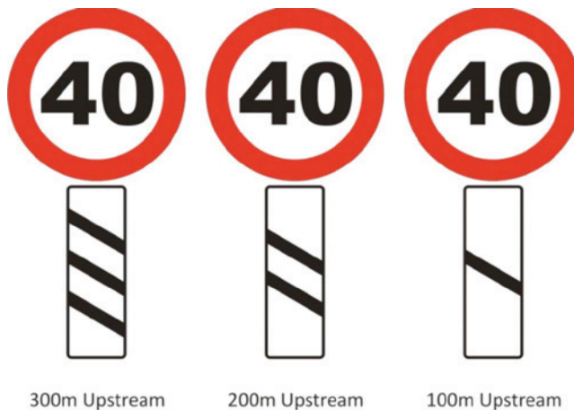
FIGURE 4 Countdown speed signs [Source: Barker and Helliari-Symons (1997)].
